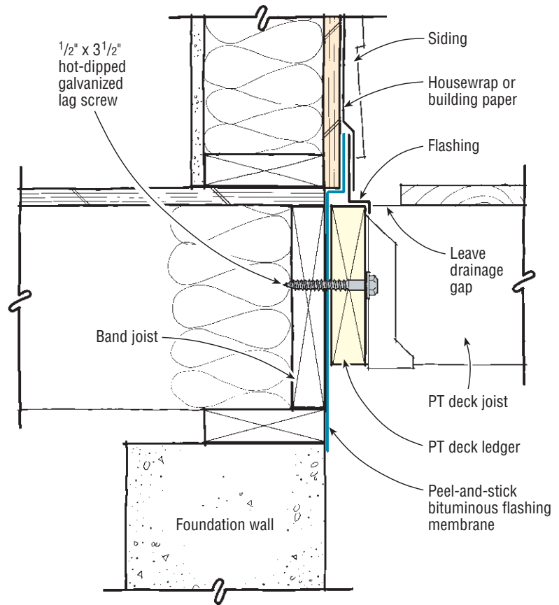
Detail 1 Fastener Schedule*
